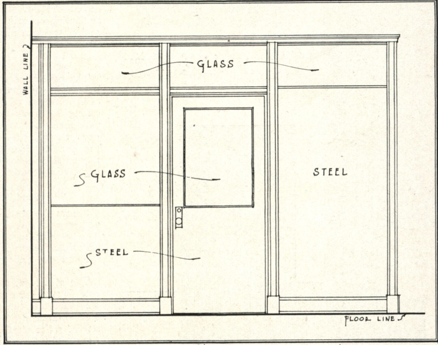
ELEVATION OF 1 3/4" INSULATED PANEL'S
