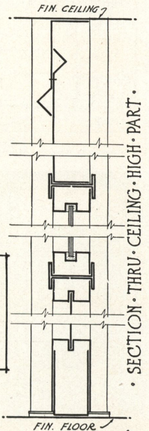
Mills Metal Commercial Partitions Steel and glass—note exceptional height
