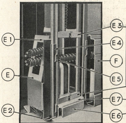
Figure 10 Base Clip
