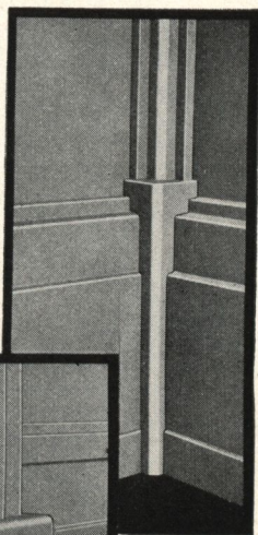
Figure 3 A close-up of the inside corner plinth showing how it fits over the base and corner mold.
