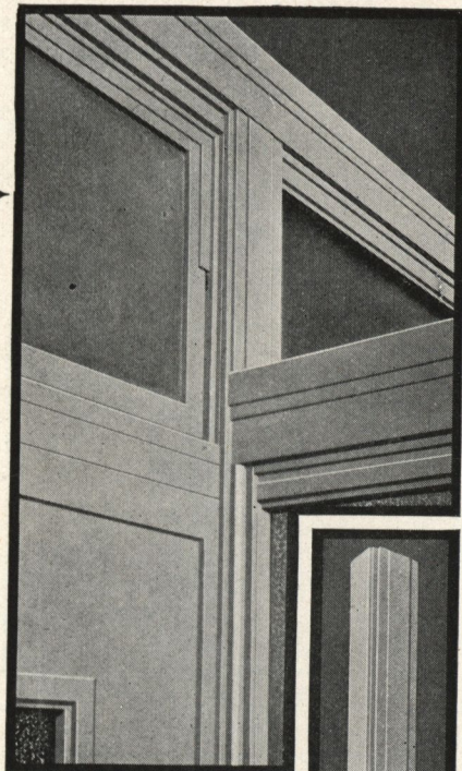
Figure 5 Shows partitions of two different cornice heights joining. Note how the lower cornice frames into the standard posts with the appearance of being specially built, although it is all built out of standard sections. Notice the adjustment over the door, allowing the door to be brought down to proper relation with the floor, no matter what the floor conditions may be. The transom is operated by a concealed interior direct acting operating device, transom moves directly with the operating handle.
